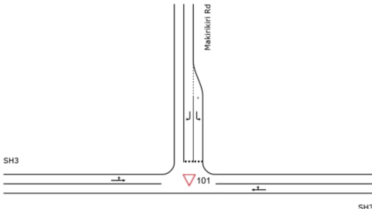
Figure 4-3: Makirikiri Road / SH3 SIDRA Intersection Layout
