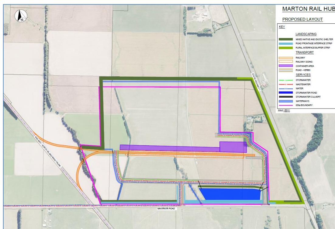
Figure O-1: Comprehensive Development Plan - Concept Plan and Layout
